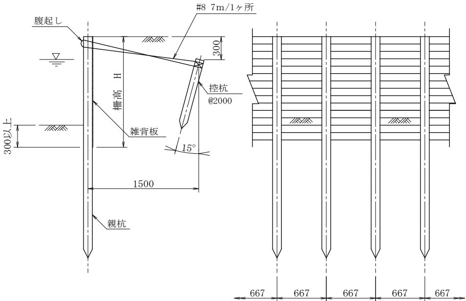
柵高 1.2m～1.5m
